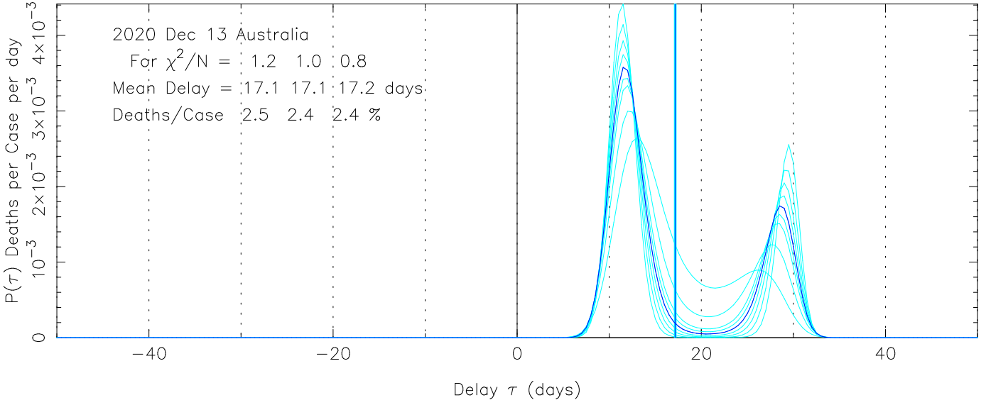
COVID-19 Delay Distribution (Deaths per Case per Day) Australia MEME fit to COVID-19 data from ECDC 2020 Dec 13
