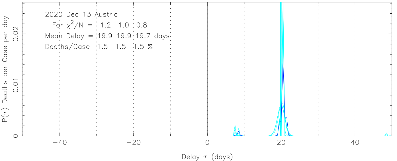
COVID-19 Delay Distribution (Deaths per Case per Day) Austria MEME fit to COVID-19 data from ECDC 2020 Dec 13
