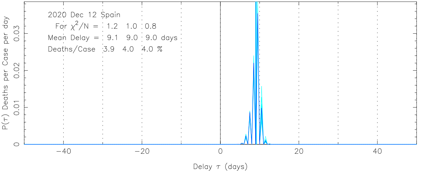
COVID-19 Delay Distribution (Deaths per Case per Day) Spain MEME fit to COVID-19 data from ECDC 2020 Dec 12
