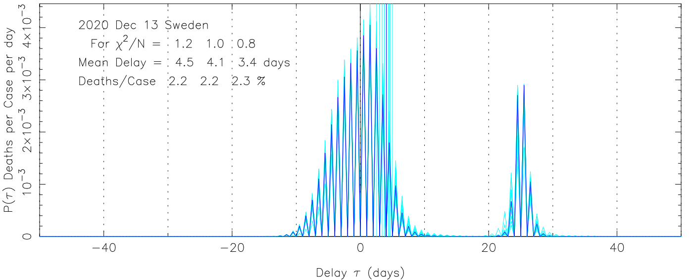
COVID-19 Delay Distribution (Deaths per Case per Day) Sweden MEME fit to COVID-19 data from ECDC 2020 Dec 13
